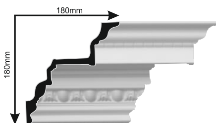
VD31G (180/180 mm x 2 m) - Skin-Tec
